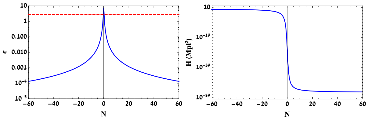
FIG. 1. The left panel shows the slow roll parameter \epsilon vs. the number of e -folds for the ansatz (1), in a logarithmic scale. The right panel shows the corresponding Hubble function of the vacuum vs. the number of e -folds.
