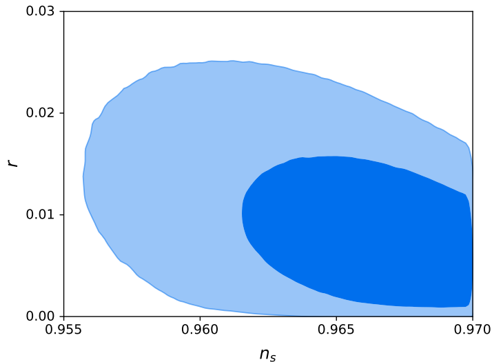
FIG. 2. The predicted scalar to tensor ratio vs. the primordial tilt of the model.
