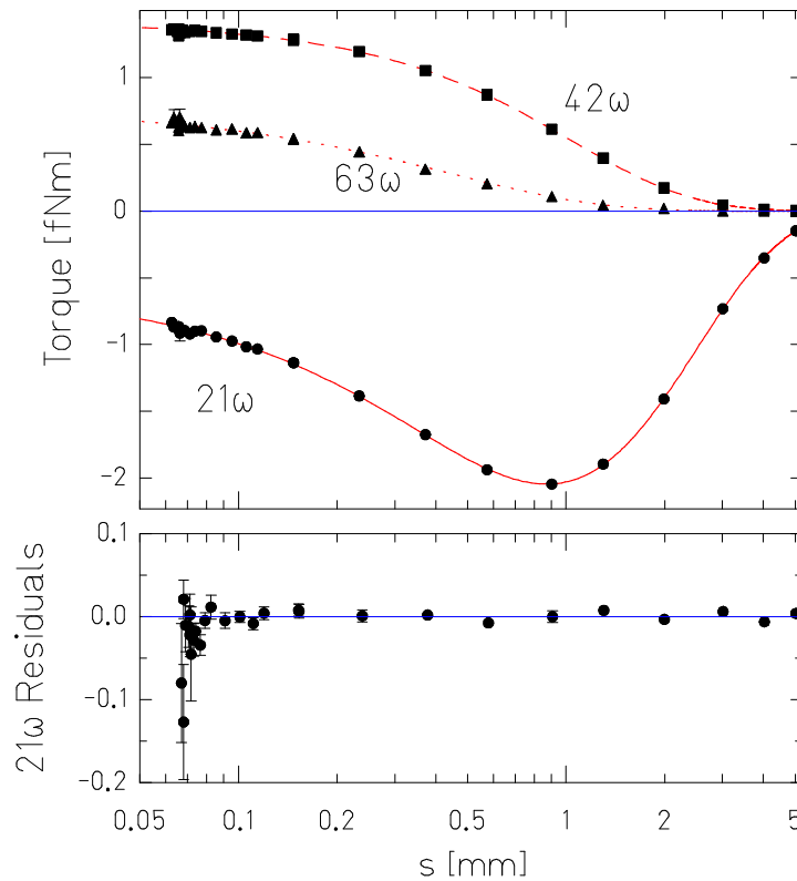
Figure 3: Top: Harmonic components of the torque on the pendulum as a function of distance above the attractor, s . Bottom: Newtonian residuals of the 21\omega torque. The agreement with the ISL is good for test mass separations above 80 \mu\text{m} ; however, we are currently investigating the small discrepancy at very short distances.
