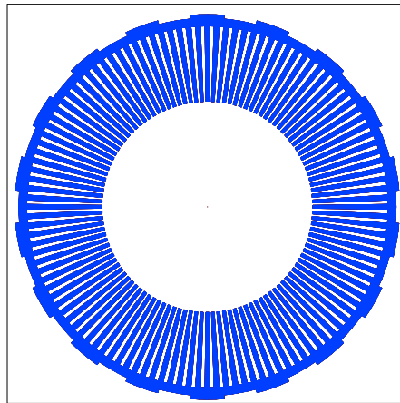
Figure 4: Top view of the active mass of the new wedge pendulum design. The 120 pendulum wedges will interact with an identical, rotating attractor mass to produce a 120\omega torque on the pendulum. The 18 wedges on the outer rim will provide an additional, long-range signal. The outer diameter of the ring is approximately 5 cm.
