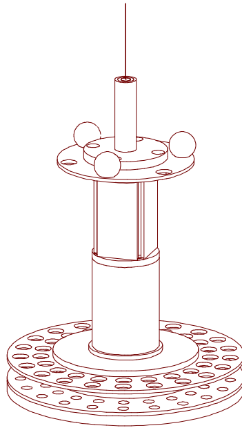
Figure 2: Eöt-Wash torsion pendulum and rotating attractor used in short-range gravity tests. The three small spheres near the top of the pendulum are used for a continuous calibration of the torque scale. The four rectangular mirrors comprise part of the angle readout system. The rotating attractor disks can be seen below the pendulum. The 10 \mu\text{m} -thick conducting membrane that separates the pendulum and attractor is omitted for clarity.
